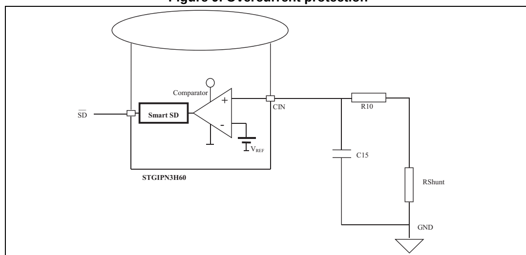
Figure 9. Overcurrent protection
