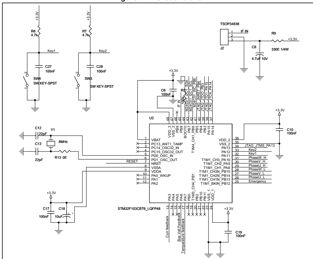
Figure 4. Microcontroller
