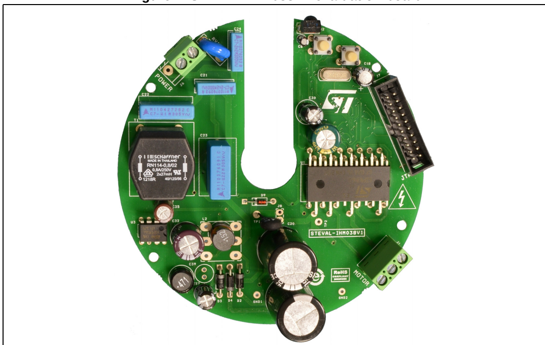
Figure 1. STEVAL-IHM038V1 evaluation board
