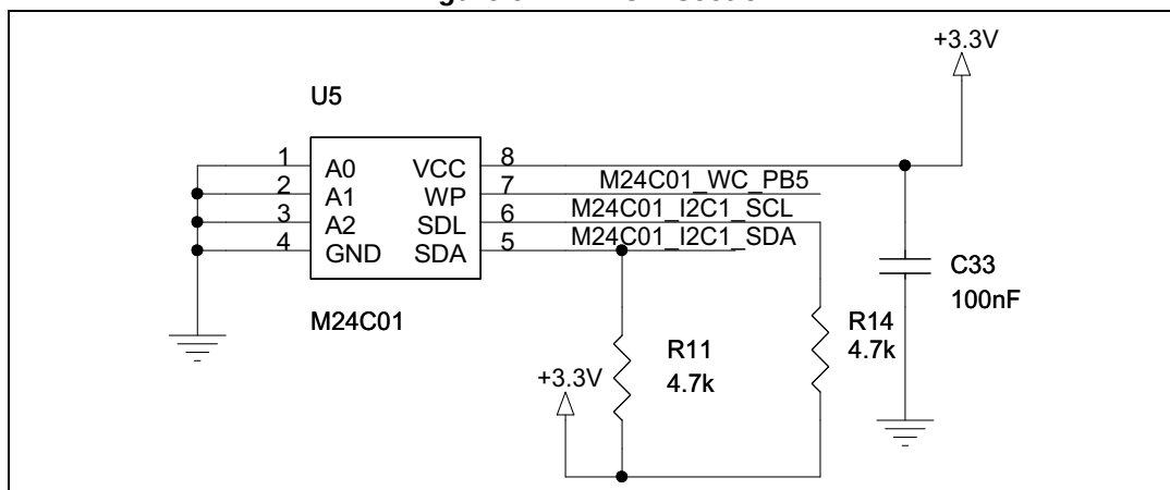
Figure 6. EEPROM section
