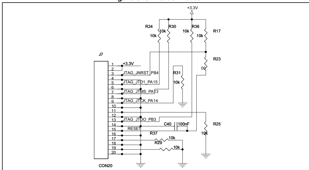
Figure 5. JTAG connector
