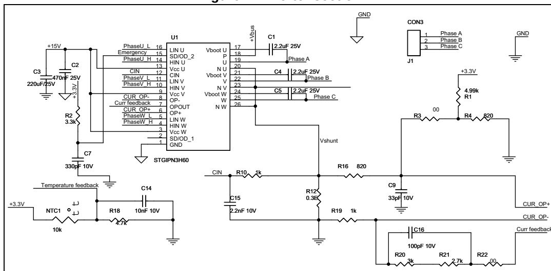
Figure 7. Inverter section
