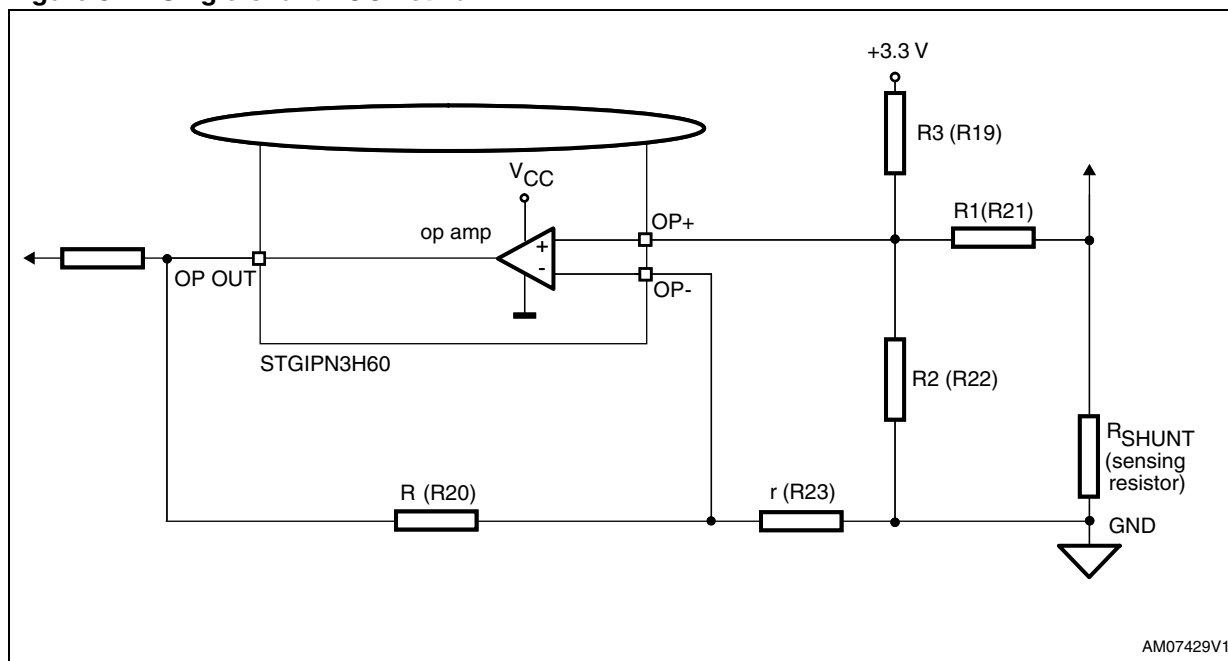
Figure 8. Single-shunt FOC network
