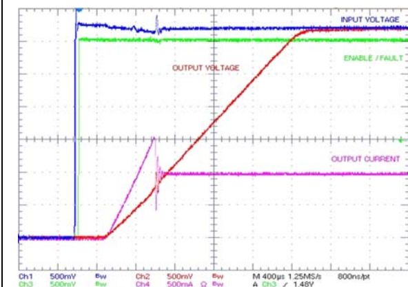
Figure 19. Thermal latch from 2 A load to short-circuit
