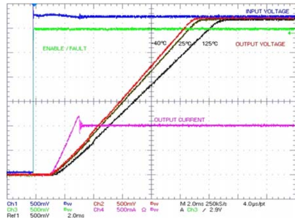
Figure 14. V_{OUT} ramp-up vs. enable
