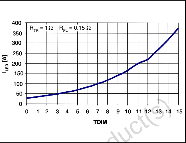
Figure 21. I_{LED} torch vs. TDIM
