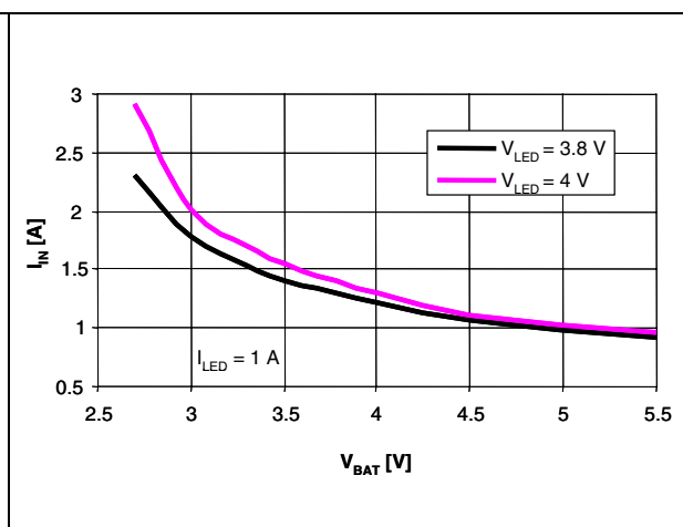
Figure 19. Input current vs. V_{BAT} ( I_{LED} = 1 A)
