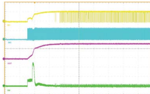
Figure 22. Startup after enable @ V_{IN}=3.6\text{ V}
