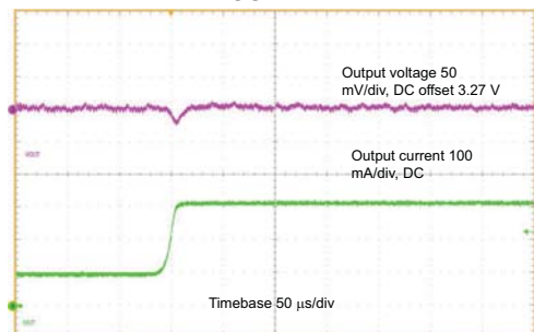
Figure 17. Load transient response @ V_{IN}=3.6\text{ V} , I_{OUT} = 100\text{ to }300\text{ mA}
