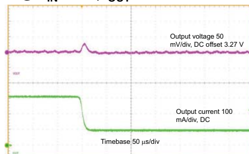
Figure 20. Load transient response @ V_{IN}=5.5\text{ V} , I_{OUT} = 300\text{ to }100\text{ mA}
