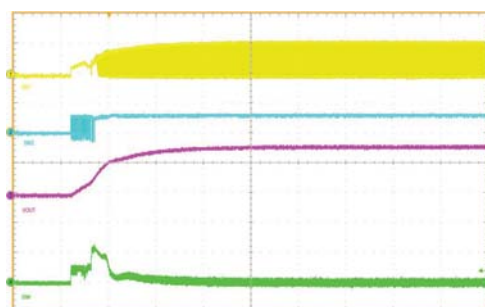
Figure 21. Startup after enable @ V_{IN}=1.8\text{ V}
