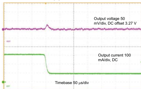
Figure 18. Load transient response @ V_{IN}=3.6\text{ V} , I_{OUT} = 300\text{ mA to }100\text{ mA}
