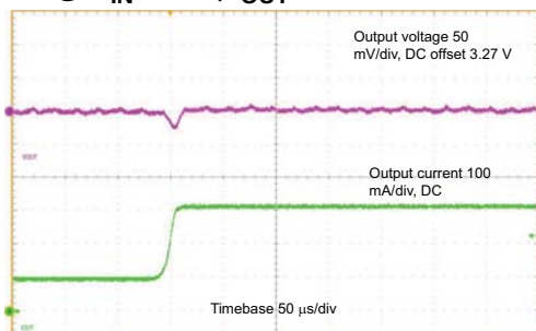
Figure 19. Load transient response @ V_{IN}=5.5\text{ V} , I_{OUT} = 100\text{ to }300\text{ mA}
