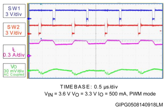
Figure 12: Buck-boost region operation @ I_O = 500 mA
