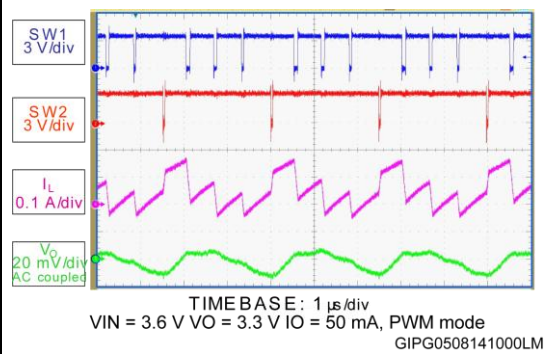
Figure 13: Buck-boost region operation @ I_O = 50 mA
