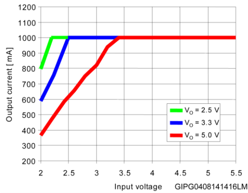
Figure 8: Max. IOUT vs. VIN
