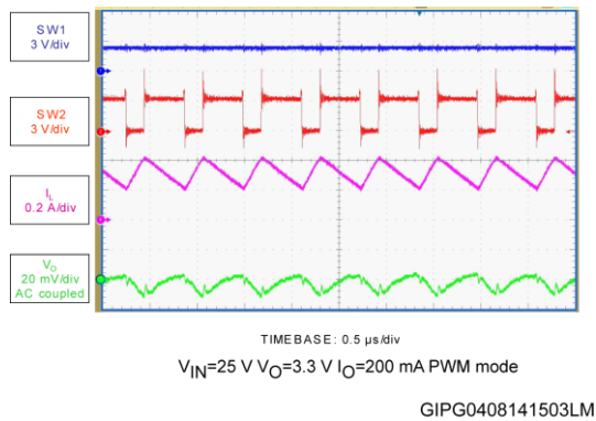
Figure 10: Boost region operation I_O = 200 mA
