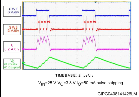
Figure 9: Boost region operation
