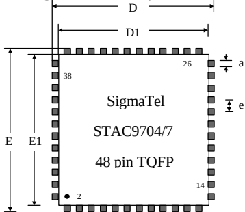
Figure 1 – Package Outline
