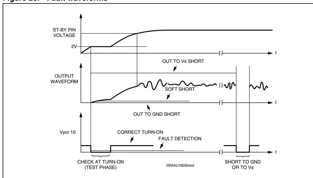
Figure 26. Fault waveforms
