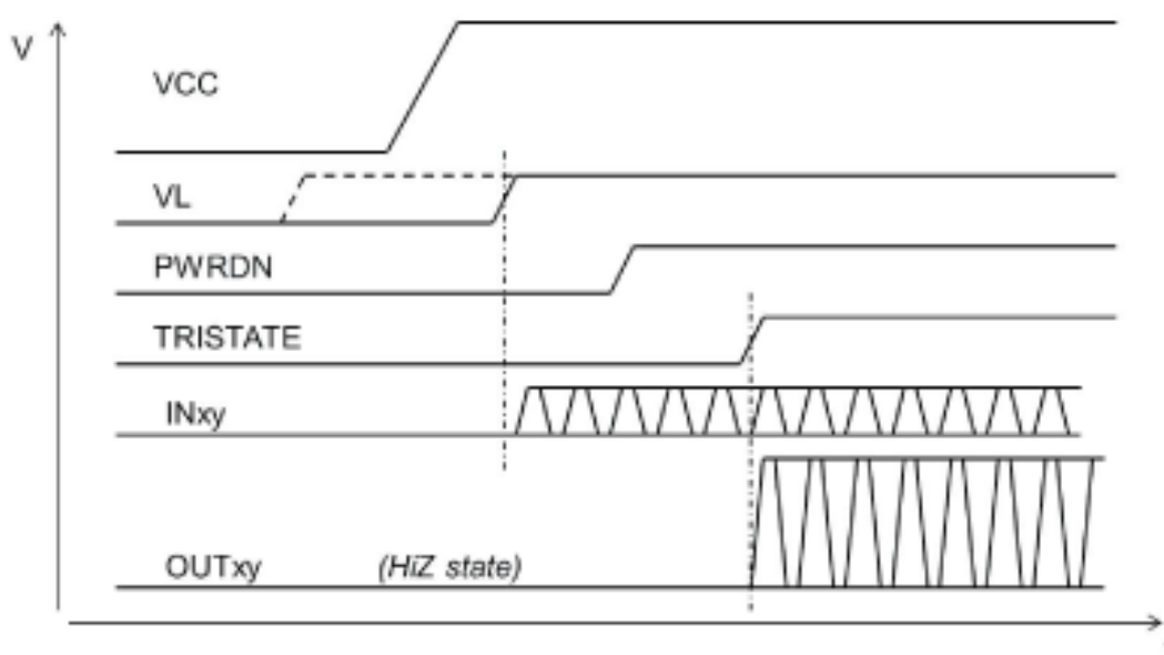
Figure 4. Power-ON sequence
