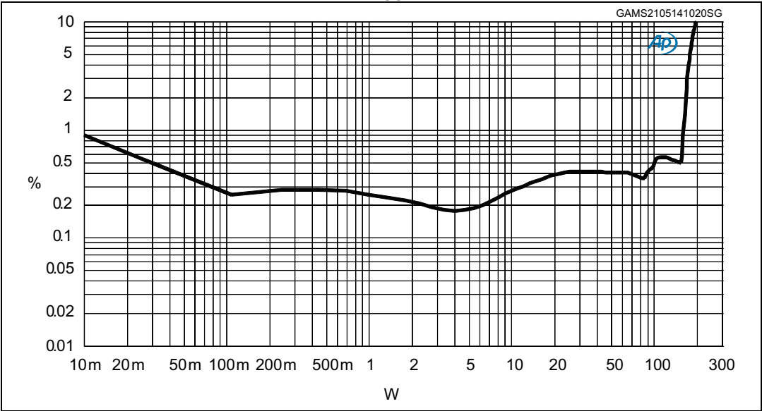
Figure 11. THD+N vs. P OUT 36V 3 Ω mono BTL
