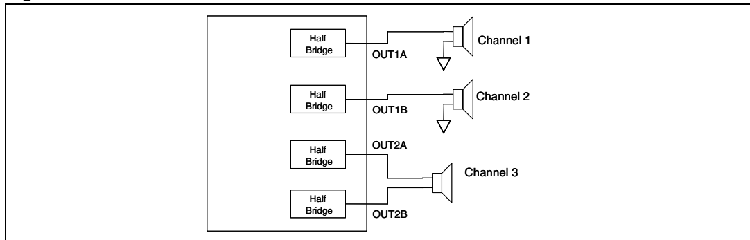
Figure 11. OCFG = 01
