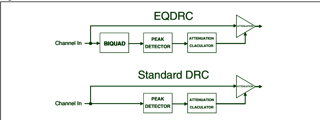
Figure 20. EQDRC scheme
