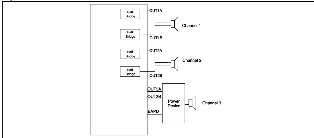
Figure 12. OCFG = 10
