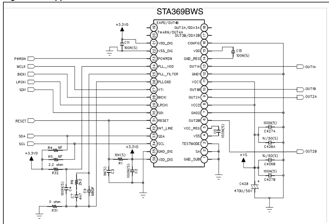
Figure 27. Applications circuit
