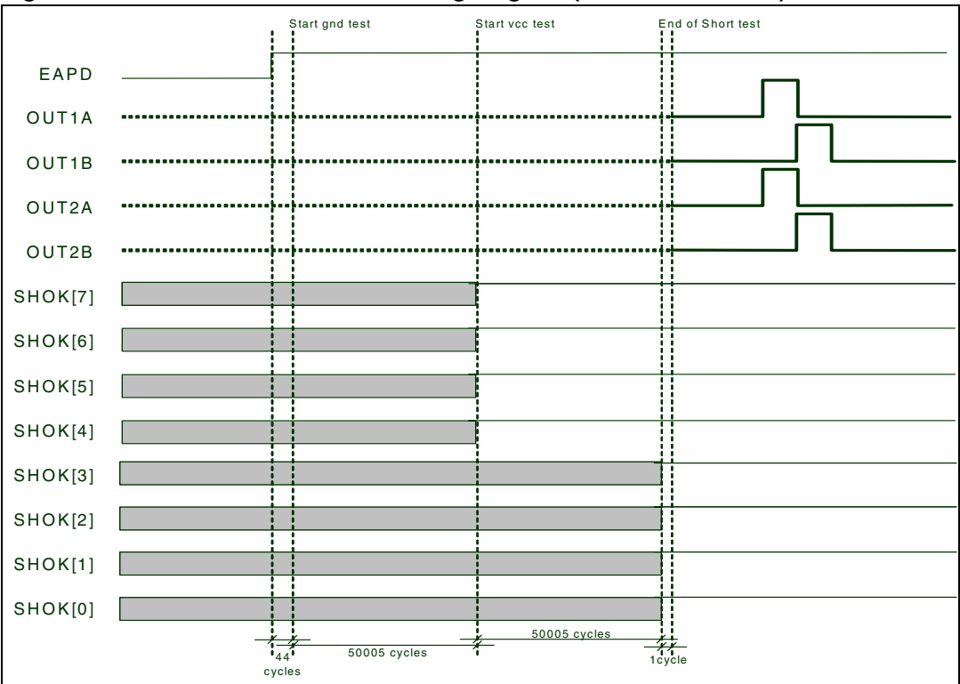
Figure 22. Short-circuit detection timing diagram (no short detected)
