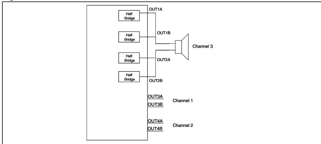
Figure 13. OCFG = 11
