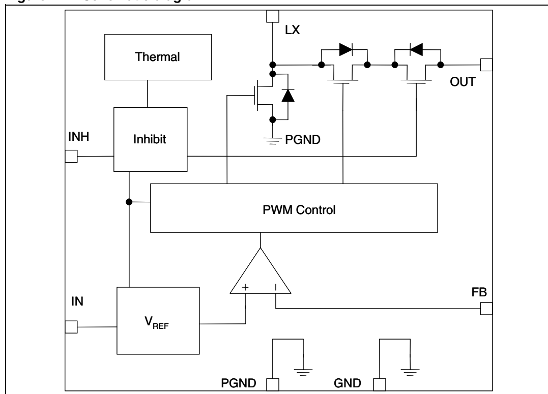
Figure 1. Schematic diagram
