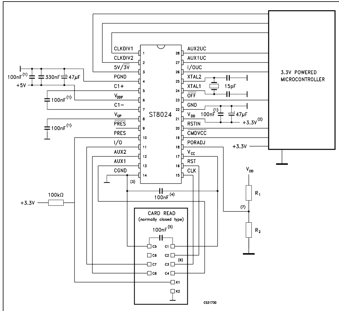
Figure 10. Application diagram
