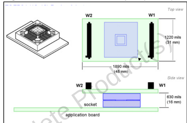
Figure 2. TQFP64 device adapter (DB583)
