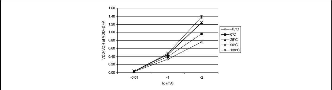
Figure 76. Typical V_{DD}-V_{OH} at V_{DD} = 2.4V
