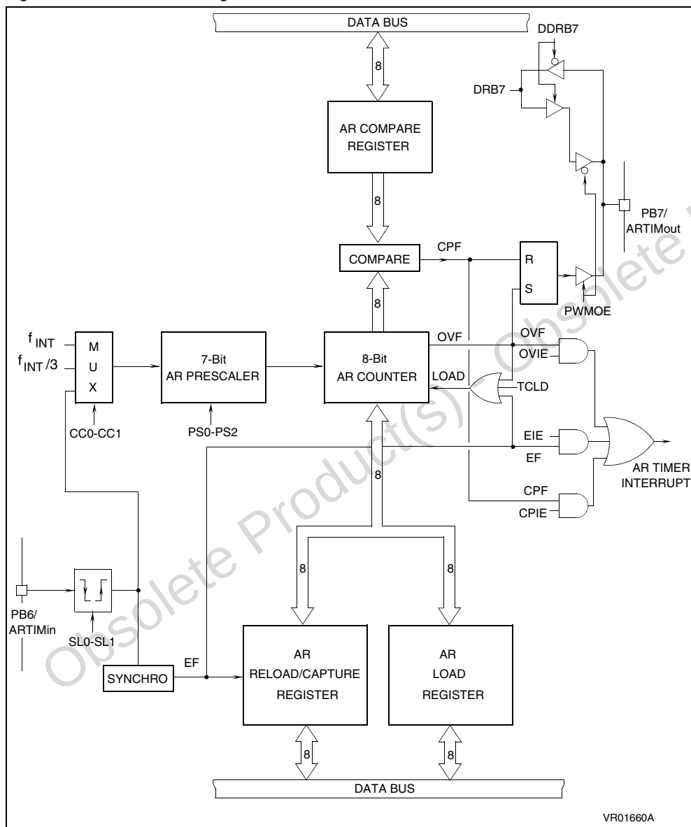
Figure 27. AR Timer Block Diagram
