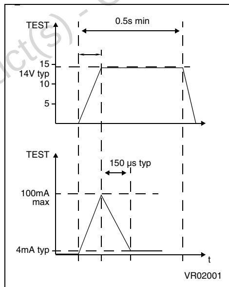
Figure 1. Programming Waveform
