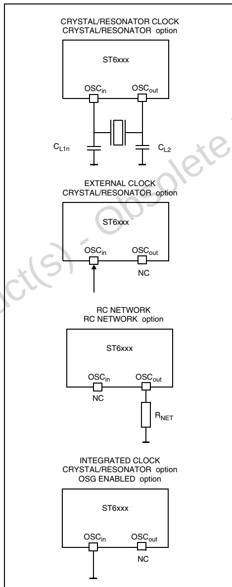
Figure 8. Oscillator Configurations
