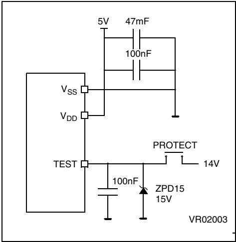
Figure 50. Programming Circuit
