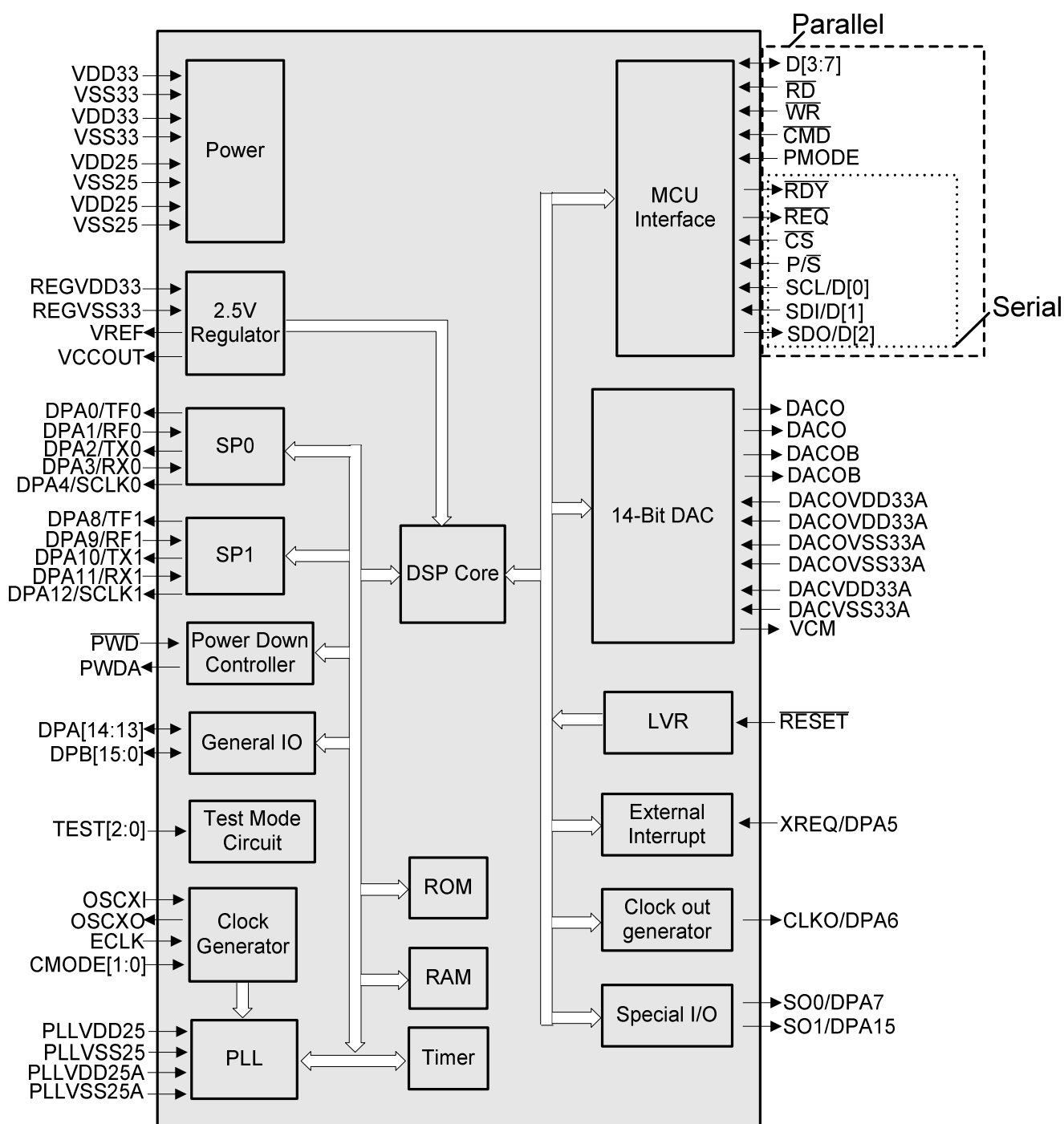
Figure 2-1 ST3003 Block Diagram
