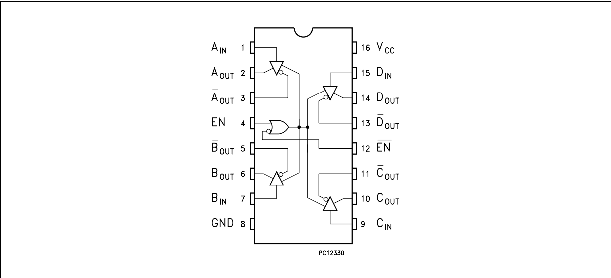
Figure 1. Pin connections
