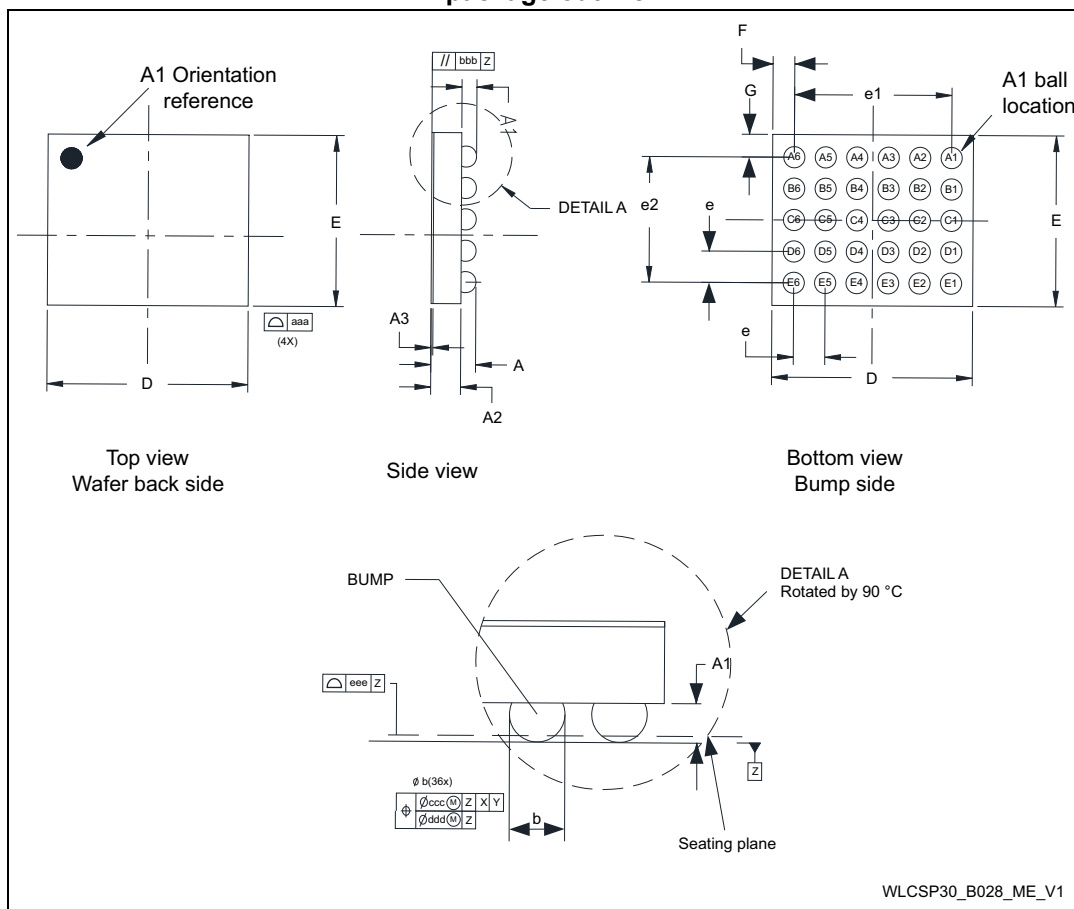
Figure 35. WLCSP30 30-ball, 3.065 x 2.865 mm, 0.5 mm pitch wafer level chip scale package outline
