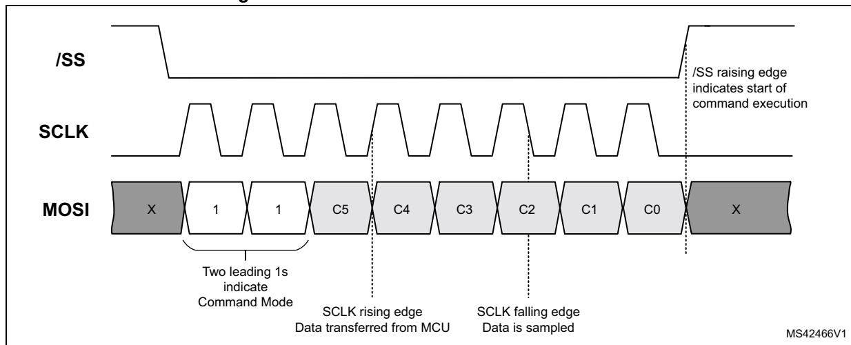
Figure 14. SPI communication: direct command
