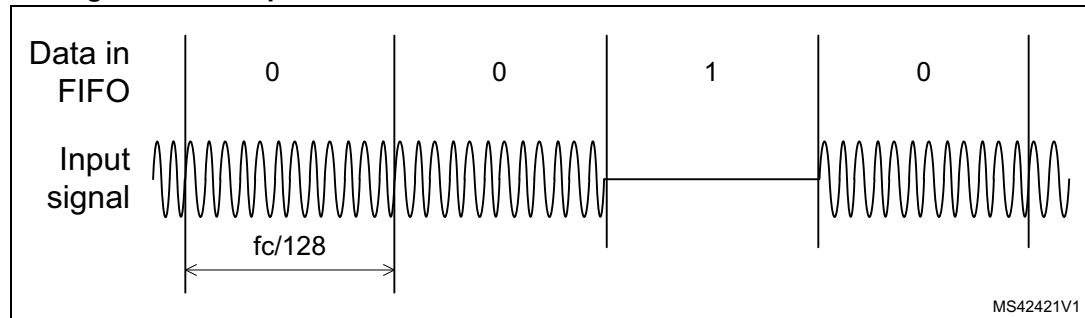
Figure 27. Example of Tx in Stream Mode for stx = 000b and OOK modulation
