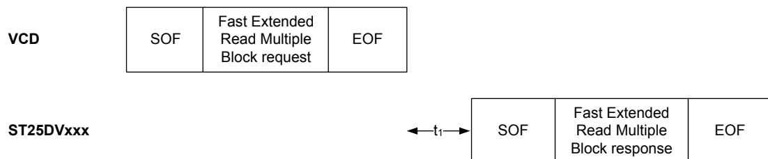
Figure 69. Fast Extended Read Multiple Block frame exchange between VCD and ST25DVxxx
