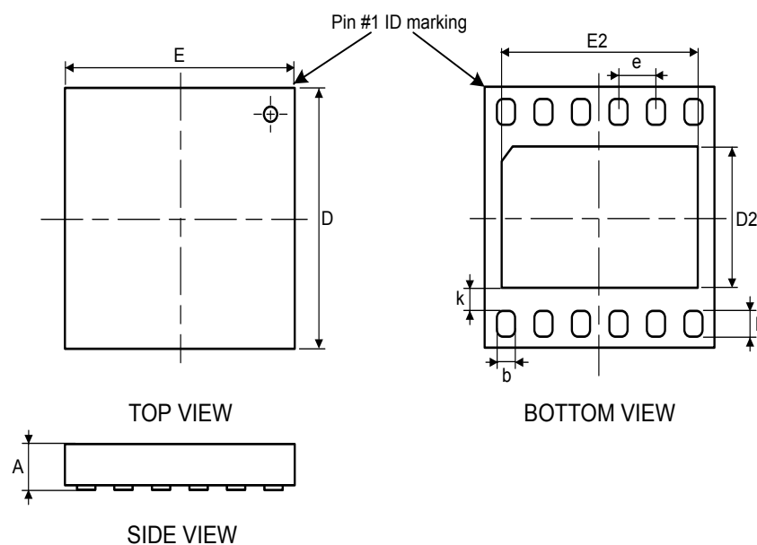
Figure 83. UFDFPN12 - 12-lead, 3x3 mm, 0.5 mm pitch ultra thin profile fine pitch dual flat package outline
