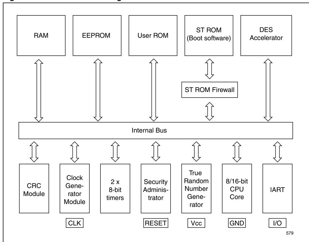
Figure 1. ST21Y036 block diagram
