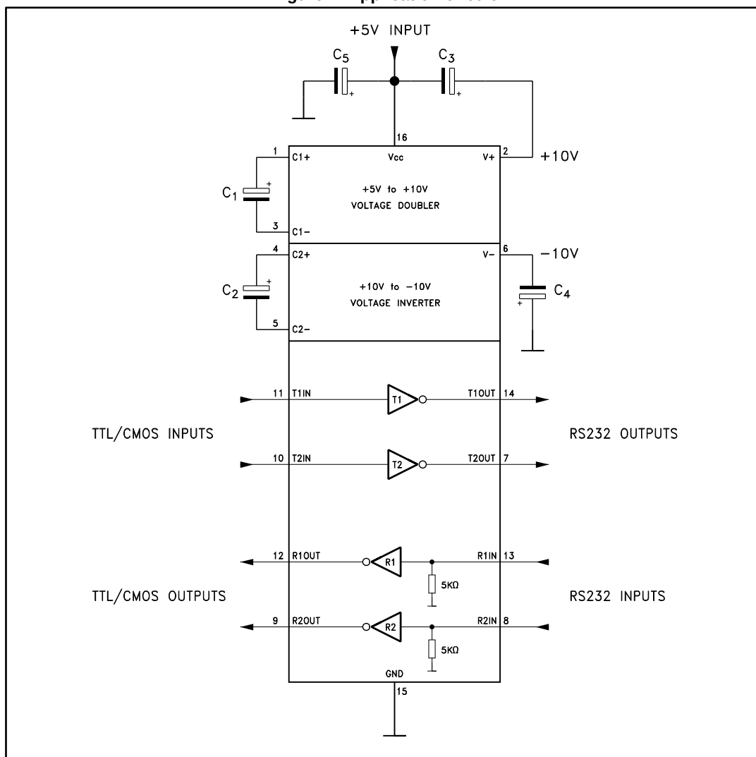
Figure 2: Application circuit
