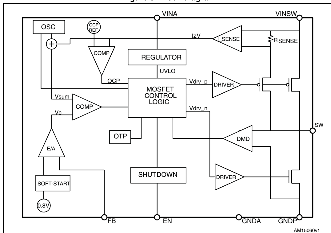
Figure 3. Block diagram
