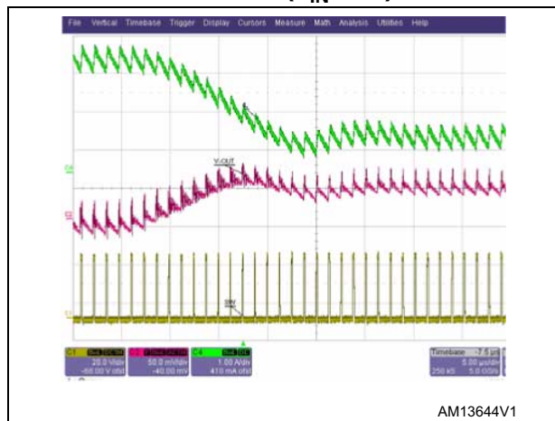
Figure 50. Zoom - 1 A to 3 A falling edge load transient ( V_{IN} 32 V)
