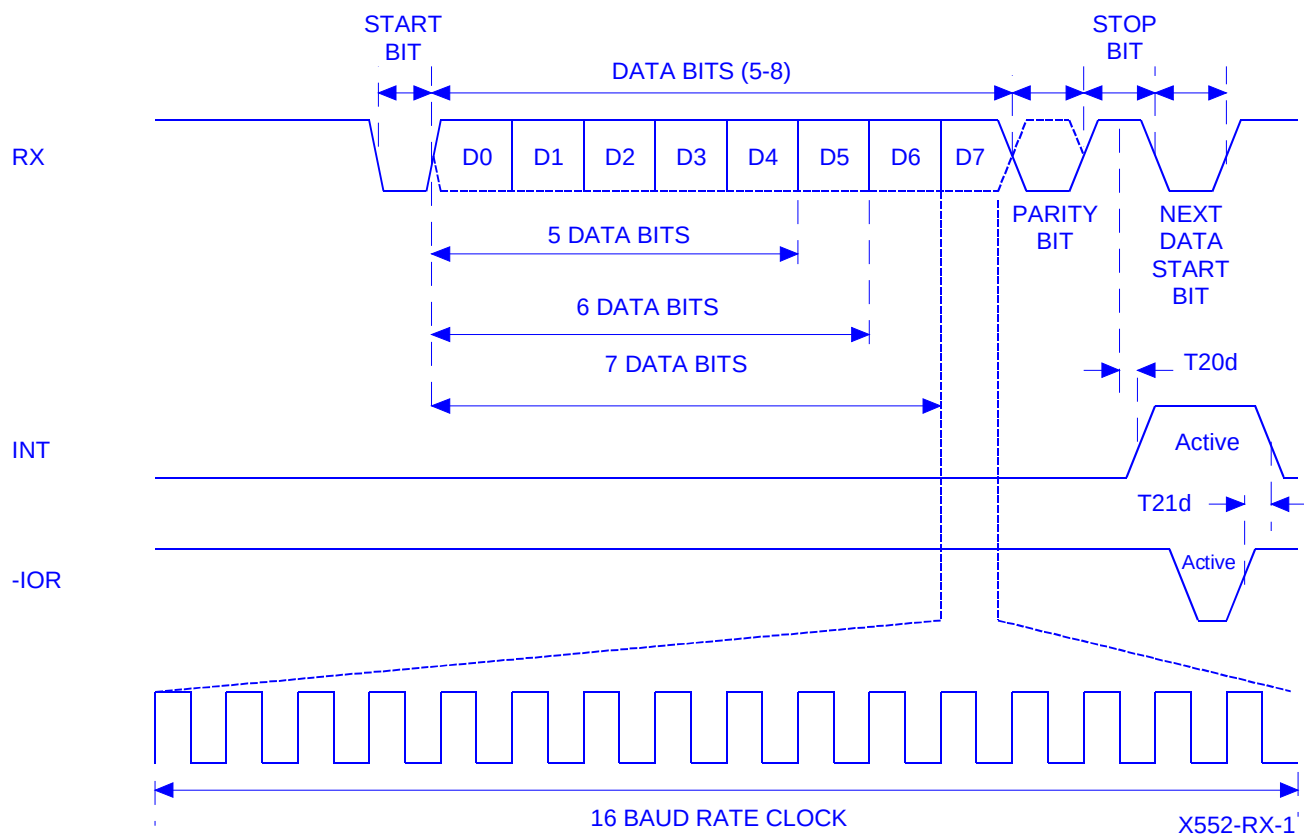
Receive timing
