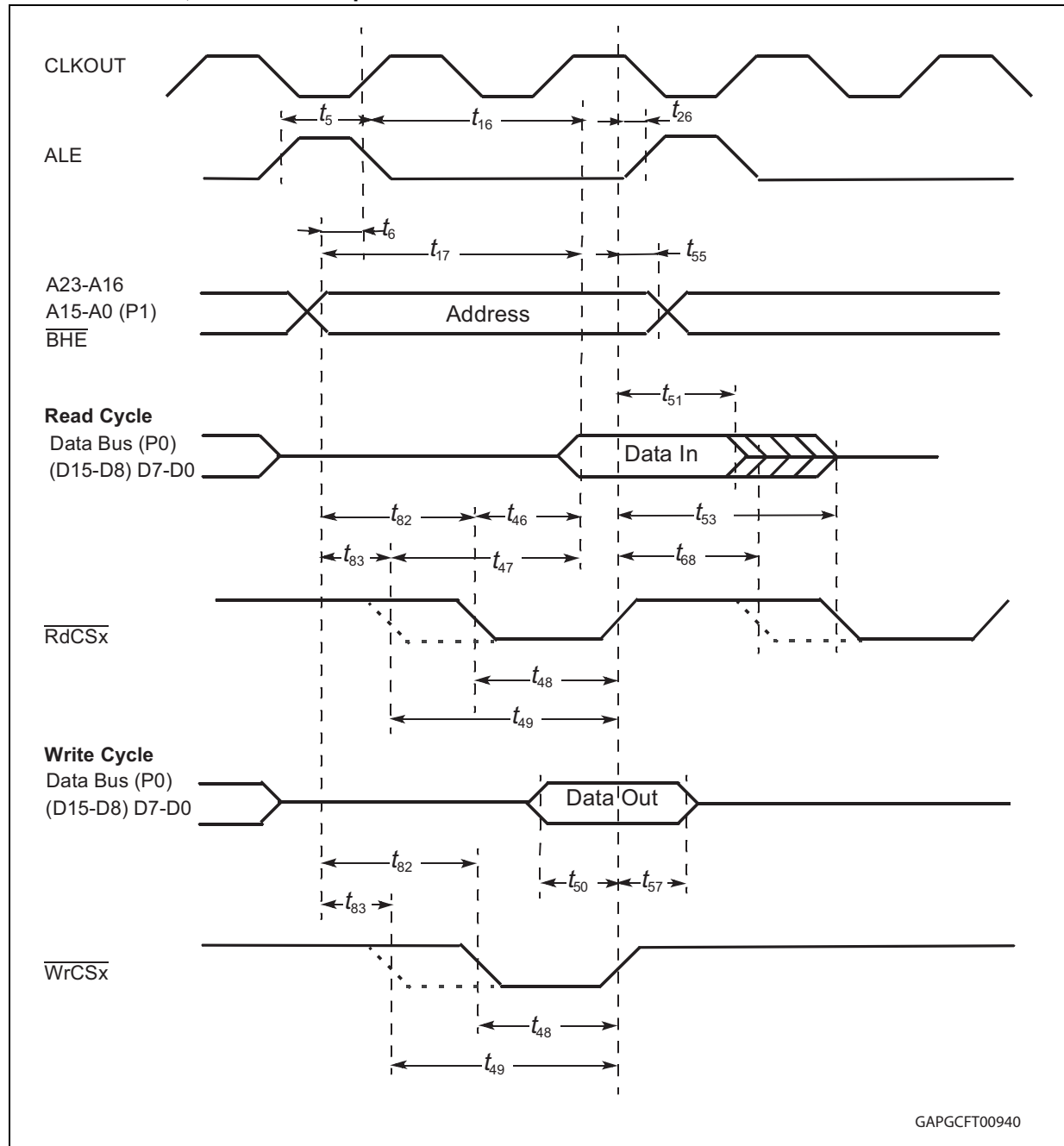
Figure 57. External memory cycle: demultiplexed bus, with/ without read/ write delay, normal ALE, read/ write chip select
