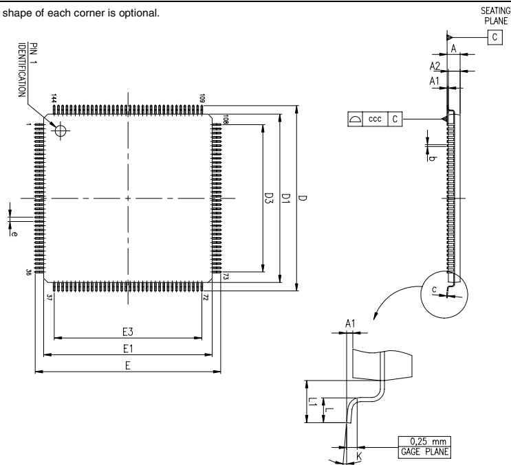
LQFP144 (20x20x1.40mm)
