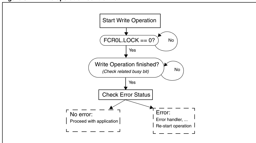
Figure 6. Write operation control flow
