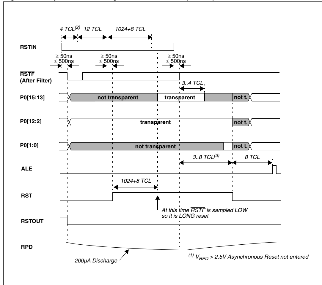
Figure 24. Synchronous long hardware RESET ( \overline{\text{EA}} = 0 )
