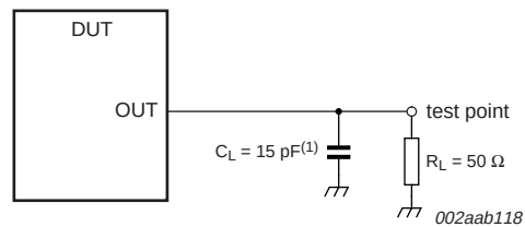
Fig 18. Load circuit, LOW-to-HIGH slew rate measurement
