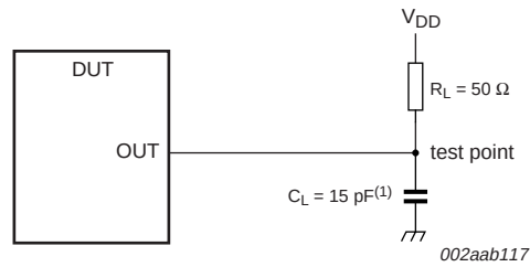
Fig 16. Load circuit, HIGH-to-LOW slew rate measurement
