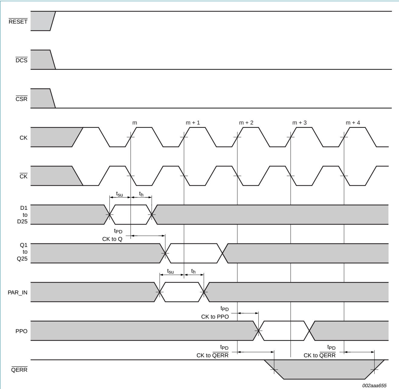
Fig 7. Timing diagram for SSTUA32866 used as a single device; C0 = 0, C1 = 0
