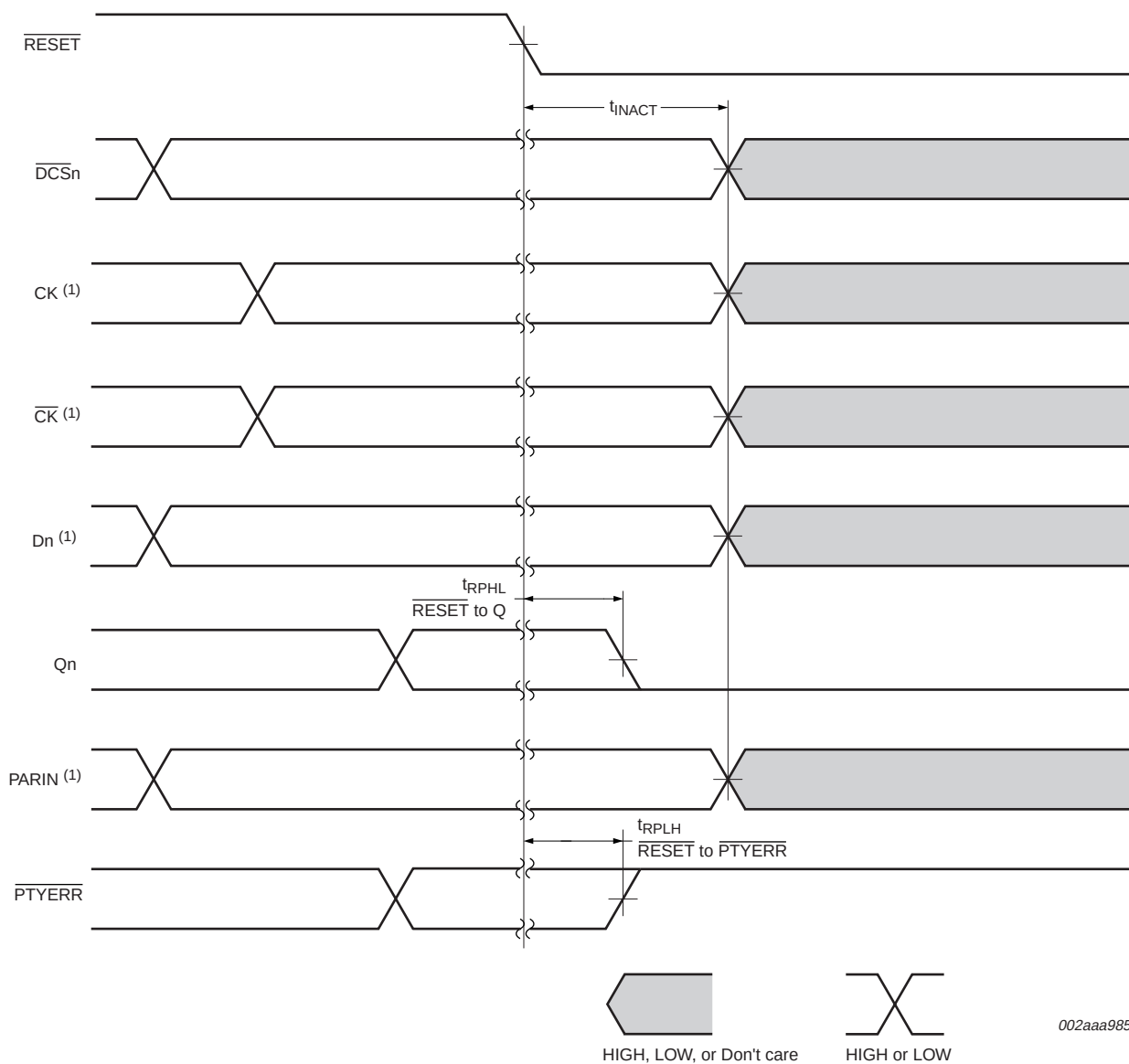
Fig 6. \overline{\text{RESET}} switches from HIGH to LOW
