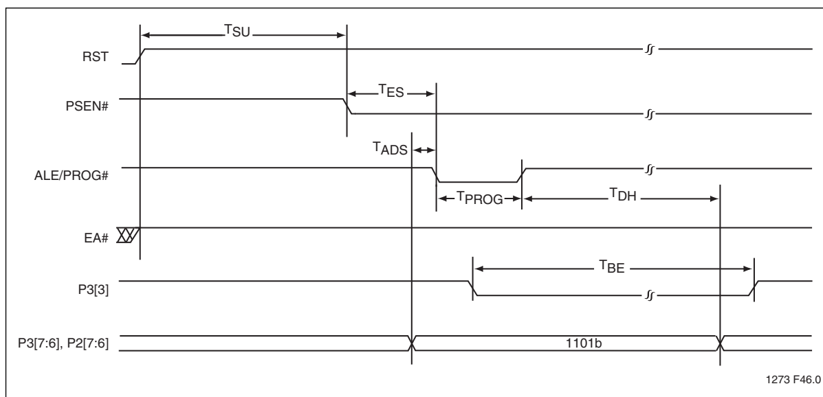
Figure 6: Block-Erase
