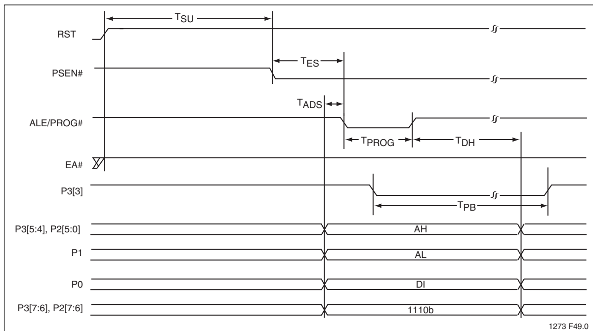
Figure 8: Byte-Program
