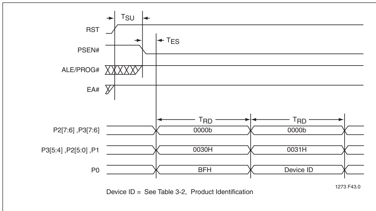
Figure 3: Read-ID
