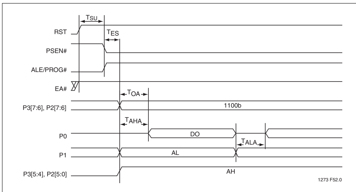
Figure 11:Byte-Verify
