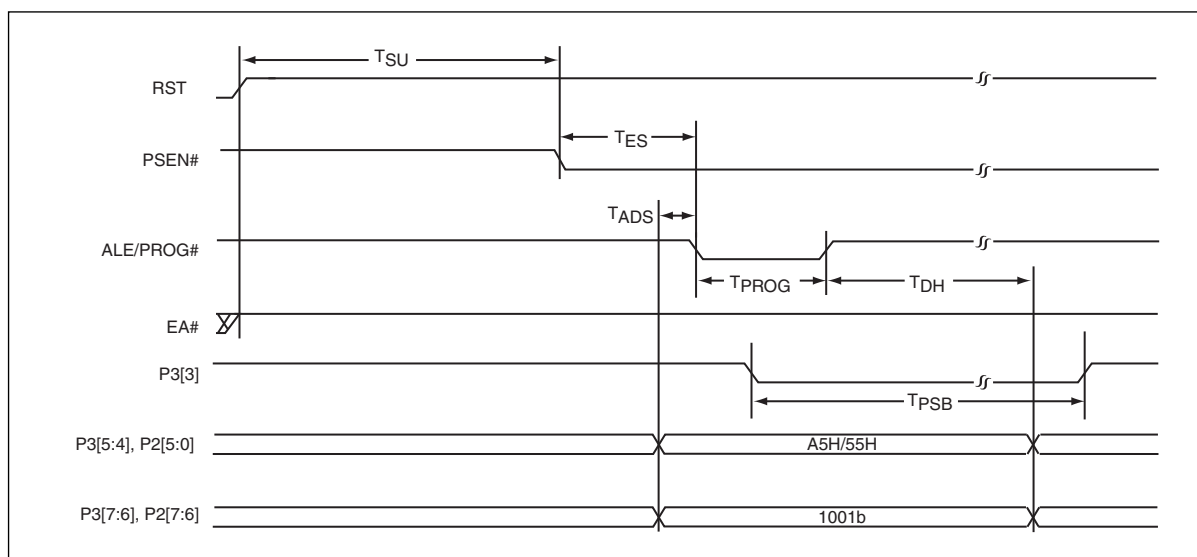
Figure 4: Select-Block1 / Select-Block0
