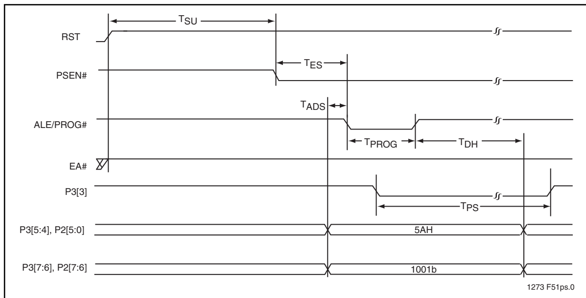
Figure 10: Prog-SC0
