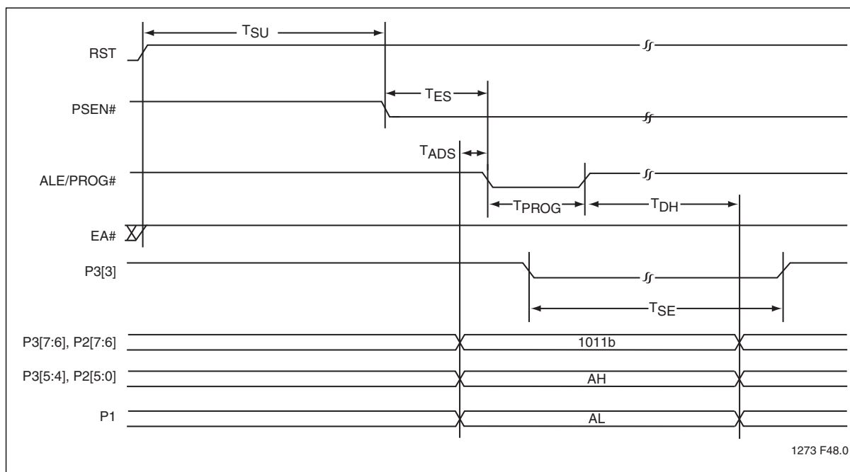
Figure 7: Sector-Erase
