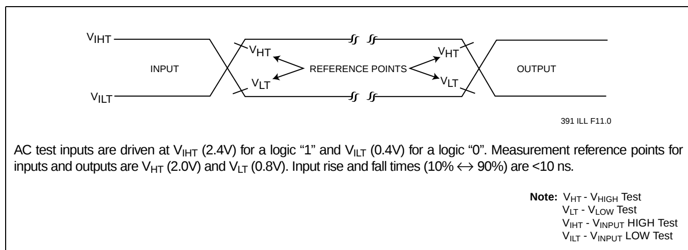
FIGURE 2-4: AC INPUT/OUTPUT REFERENCE WAVEFORMS
