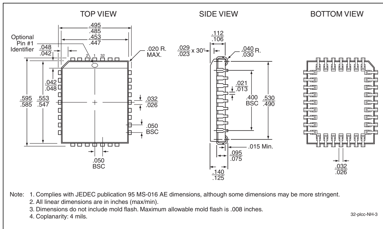
32-LEAD PLASTIC LEAD CHIP CARRIER (PLCC) SST PACKAGE CODE: NH
