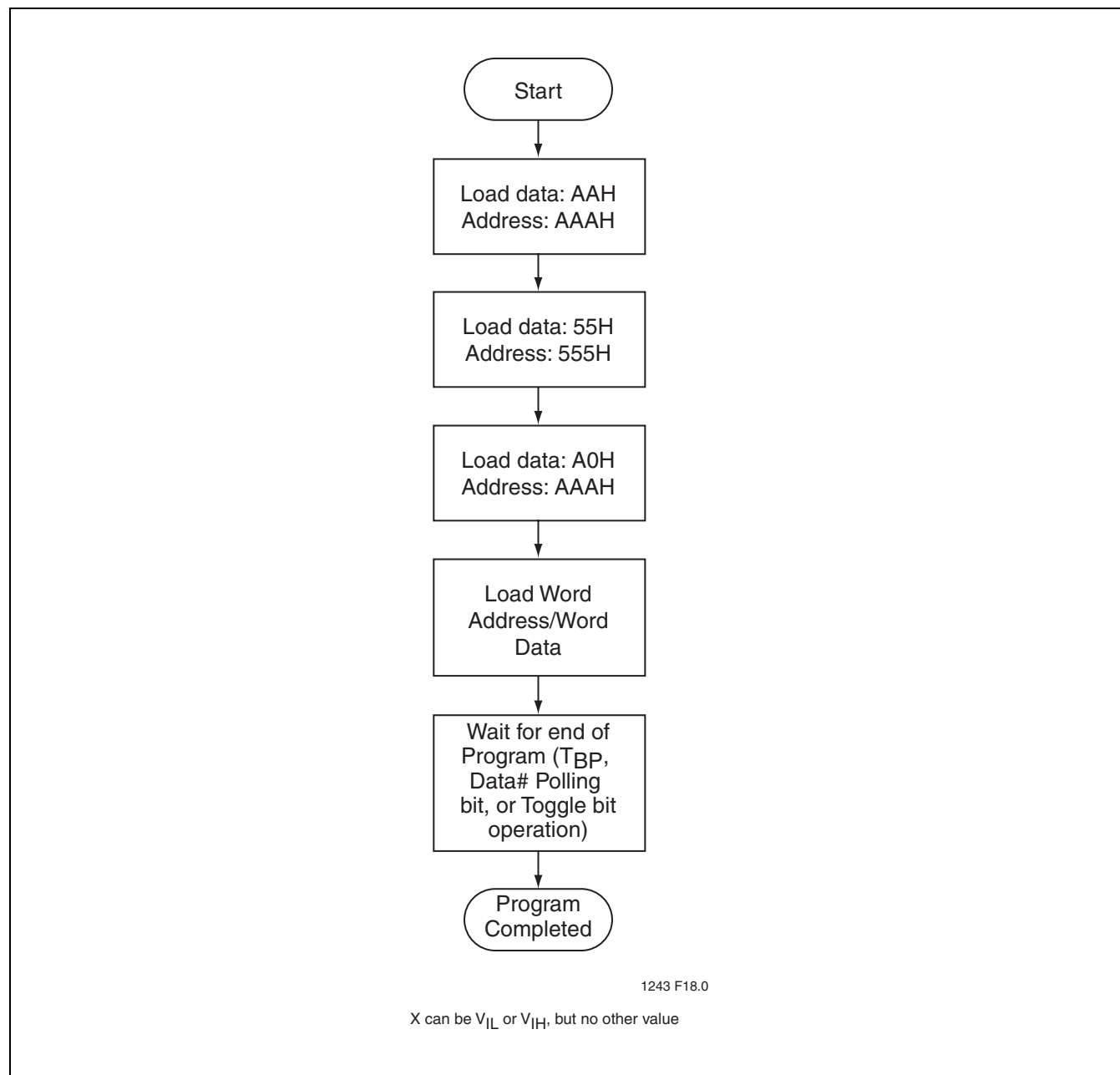
FIGURE 19: BYTE-PROGRAM ALGORITHM
