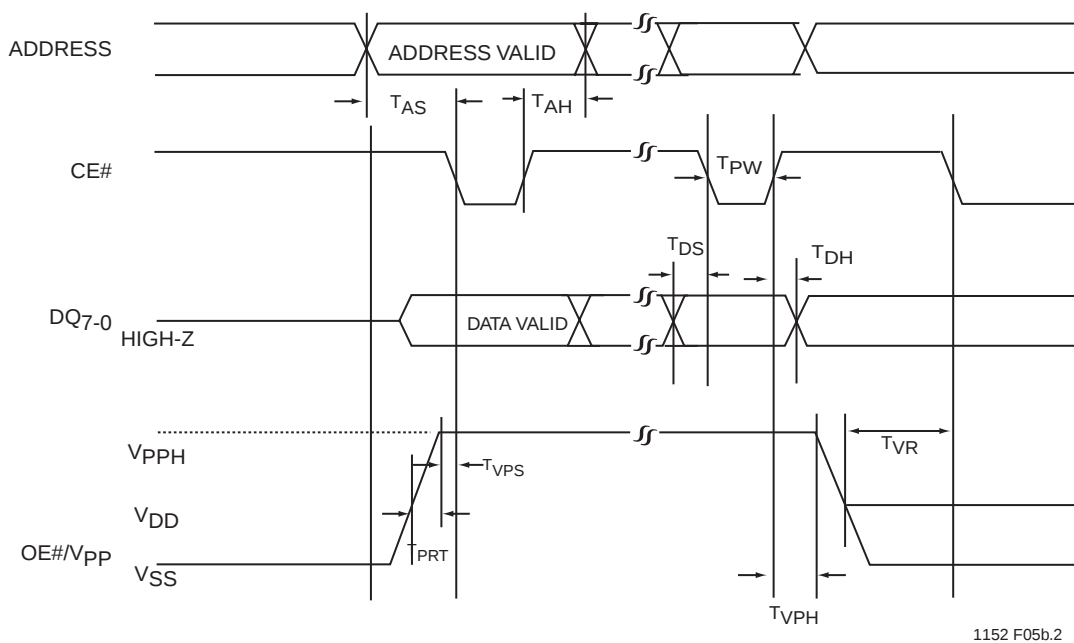
FIGURE 7: BYTE-PROGRAM TIMING DIAGRAM FOR SST27SF512
