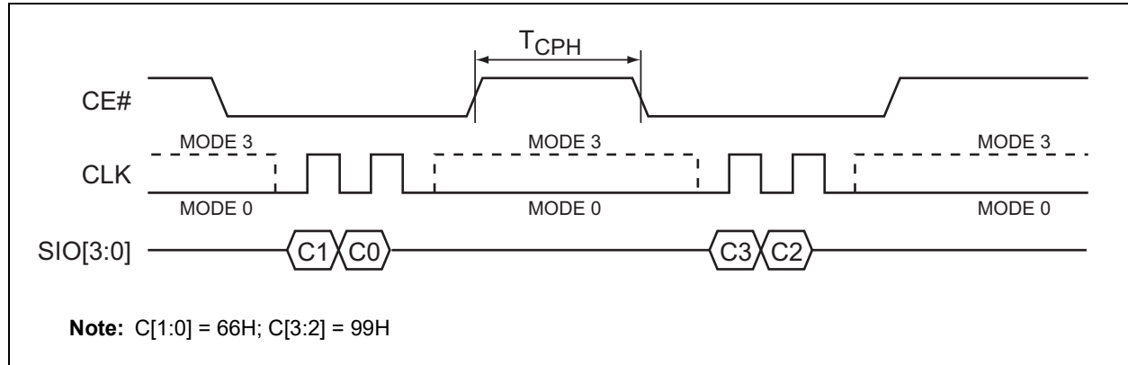
FIGURE 5-1: RESET SEQUENCE
