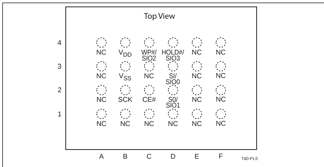
FIGURE 2-4: PIN DESCRIPTION FOR 24-BALL TBGA
