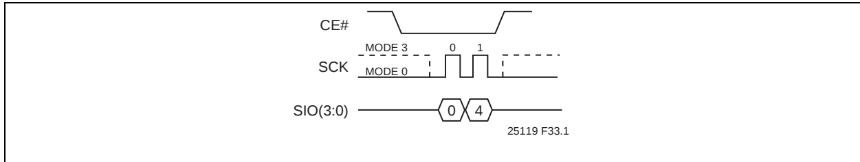
FIGURE 5-34: WRITE-DISABLE (WRDI) SEQUENCE (SIO)
