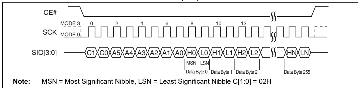
FIGURE 5-25: PAGE PROGRAM SEQUENCE (SSI)
