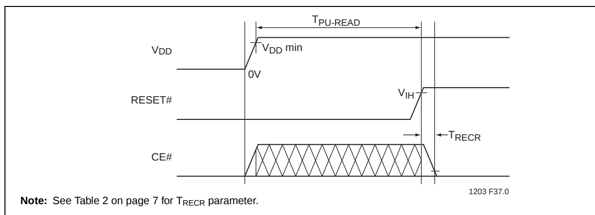
Figure 25: Power-Up Reset Diagram
