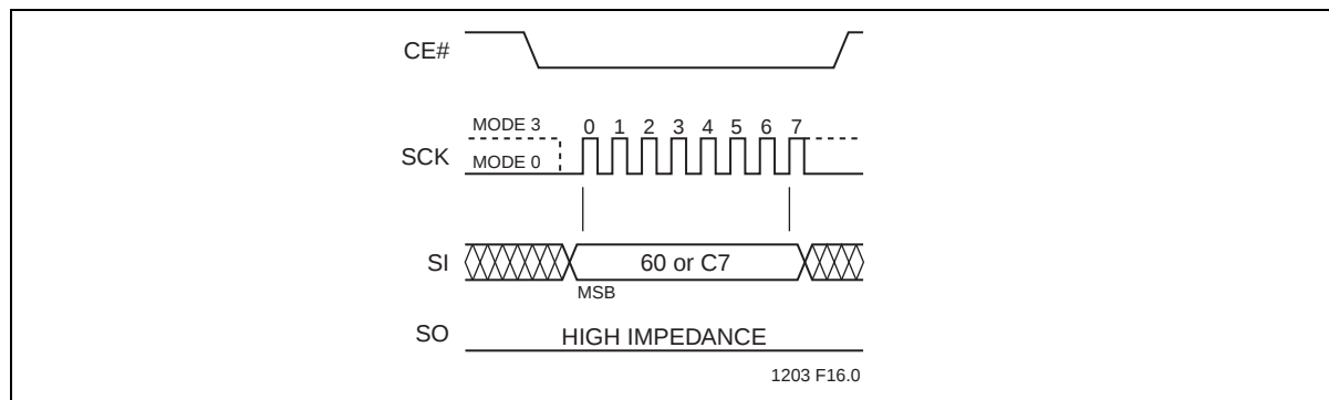
Figure 17: Chip-Erase Sequence
