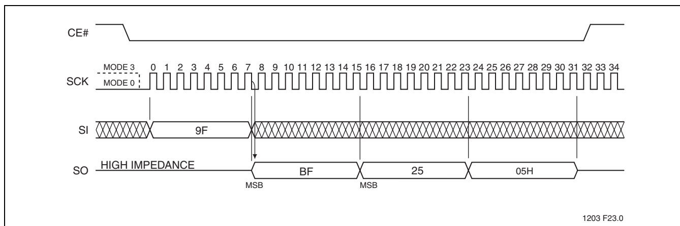
FIGURE 24: JEDEC Read-ID Sequence
