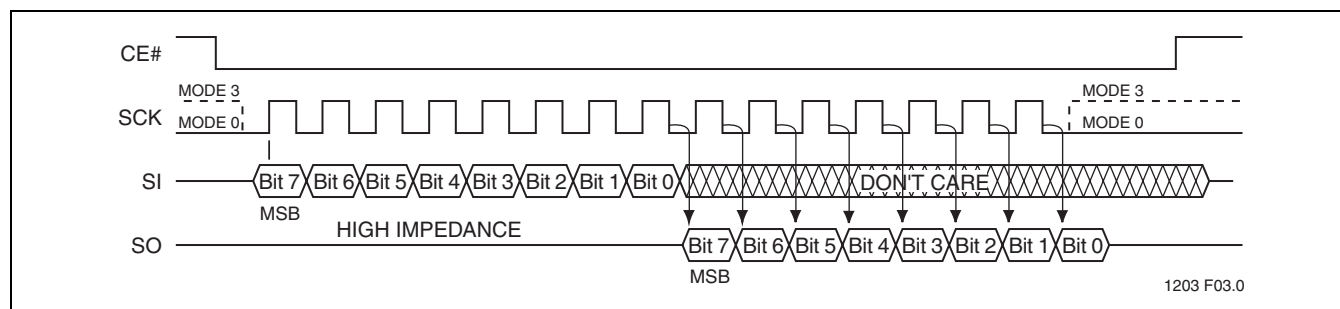
FIGURE 4: SPI Protocol
