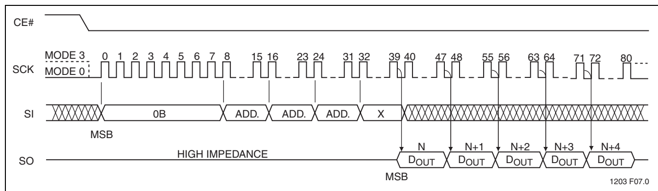
FIGURE 8: High-Speed-Read Sequence
