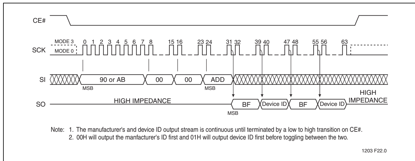
FIGURE 23: Read-ID Sequence
