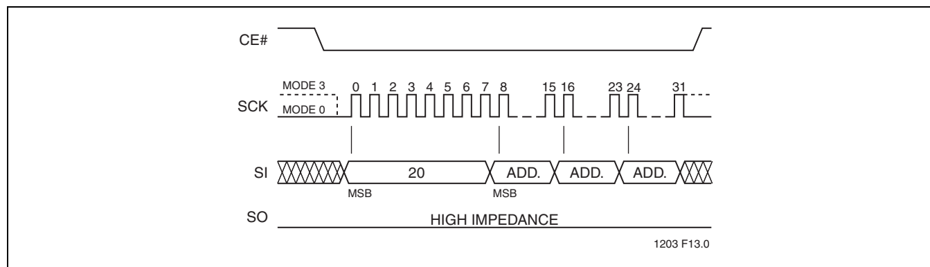
FIGURE 14: Sector-Erase Sequence
