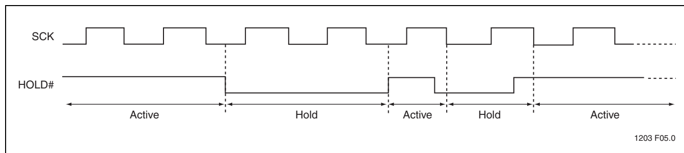
FIGURE 6: Hold Condition Waveform
