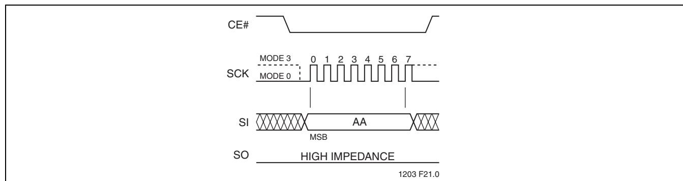
FIGURE 22: Enable-Hold Sequence
