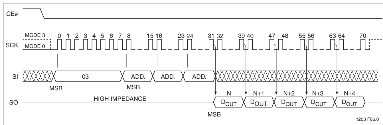
FIGURE 7: Read Sequence
