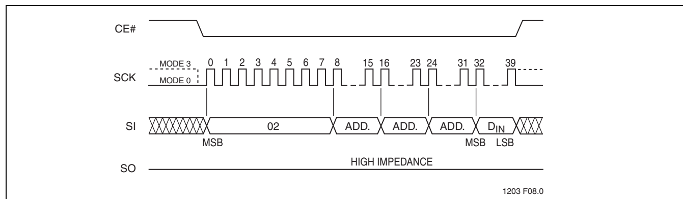
FIGURE 9: Byte-Program Sequence
