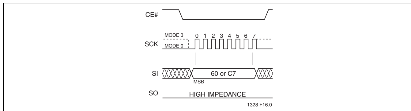
FIGURE 16: Chip-Erase Sequence
