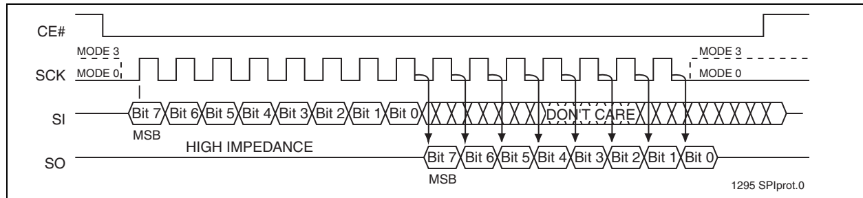
FIGURE 4-1: SPI PROTOCOL
