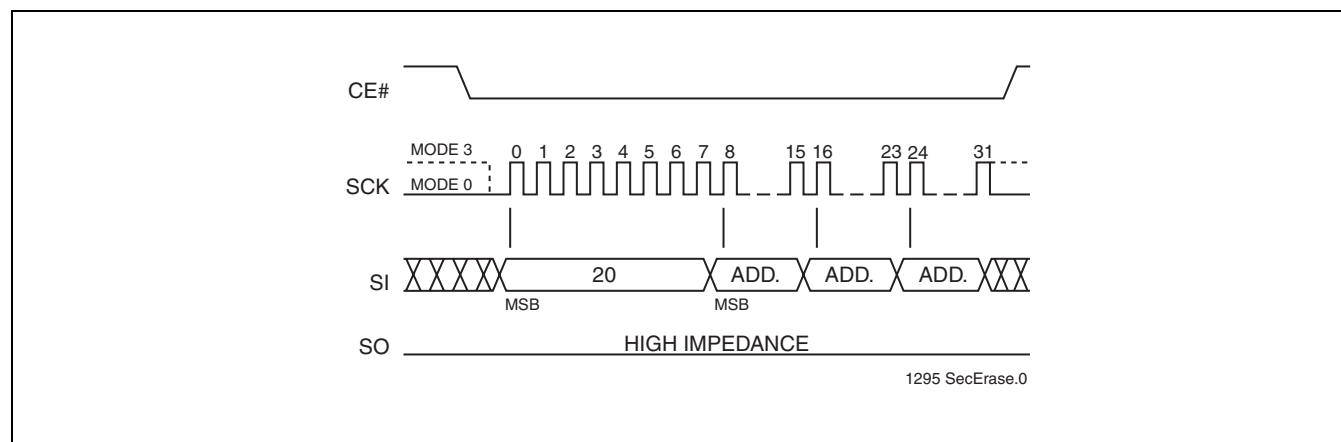
FIGURE 12: Sector-Erase Sequence
