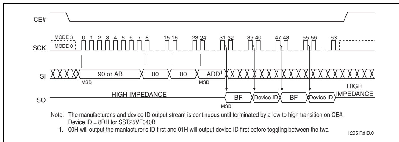
FIGURE 21: Read-ID Sequence
