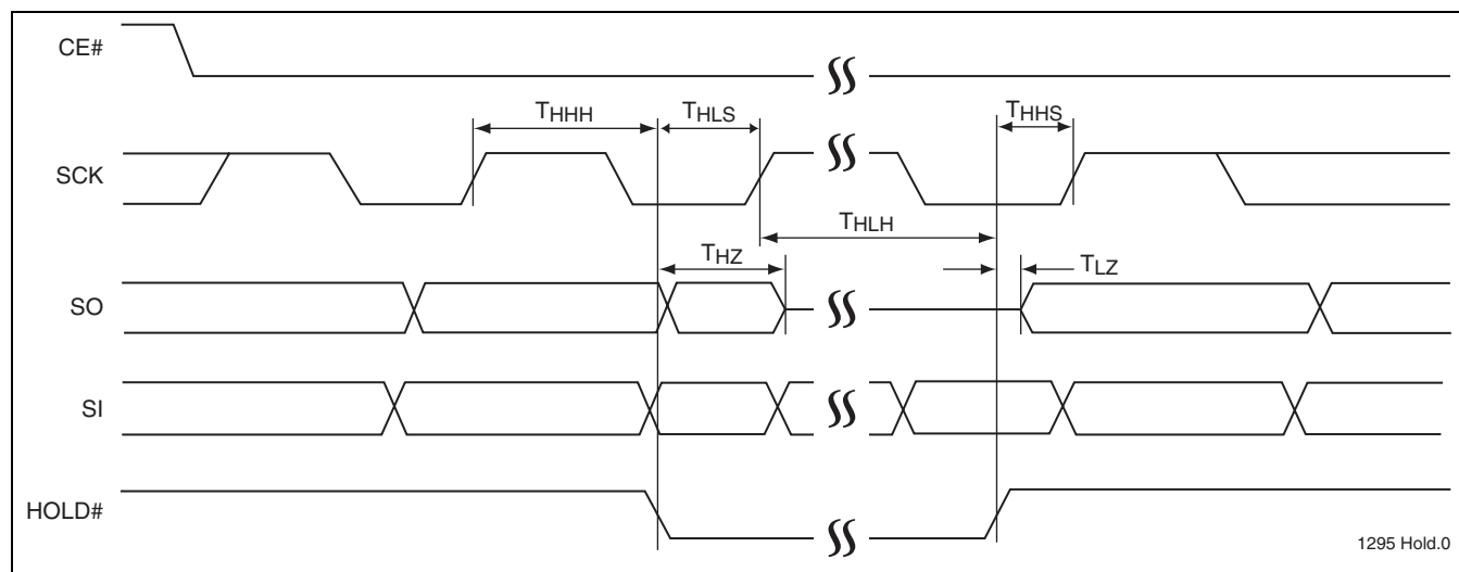
FIGURE 24: Hold Timing Diagram
