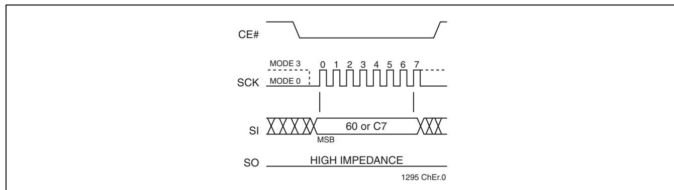
FIGURE 15: Chip-Erase Sequence
