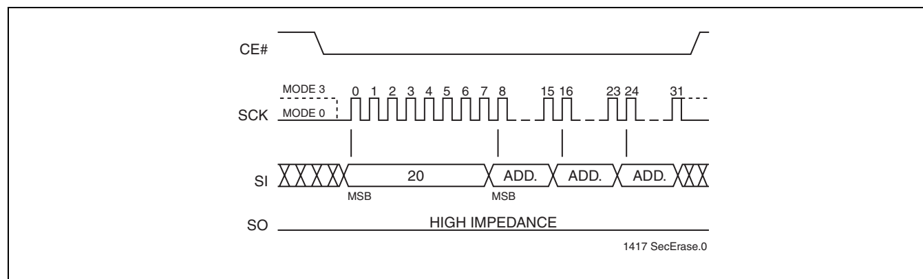
FIGURE 12: Sector-Erase Sequence
