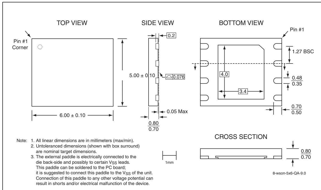
FIGURE 32: 8-Contact Very-very-thin Small Outline No-lead (WSN) SST Package Code: QA
