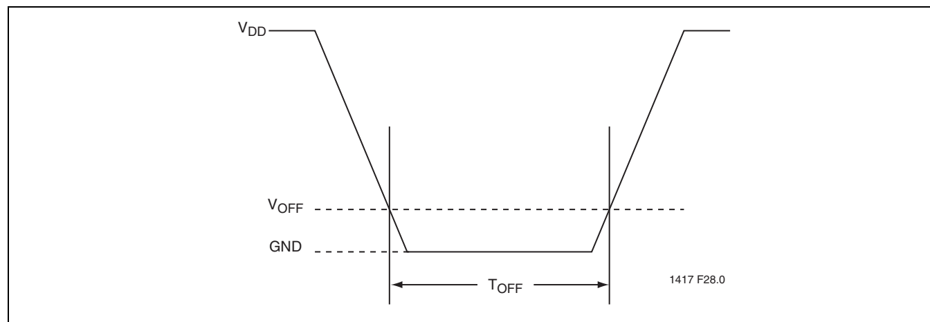
FIGURE 28: Recommended Power-up/-down Waveform
