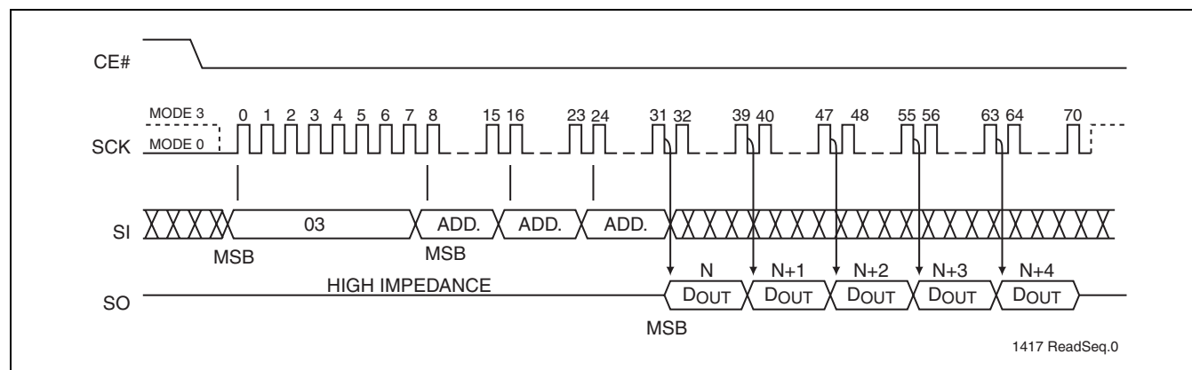
FIGURE 5: Read Sequence
