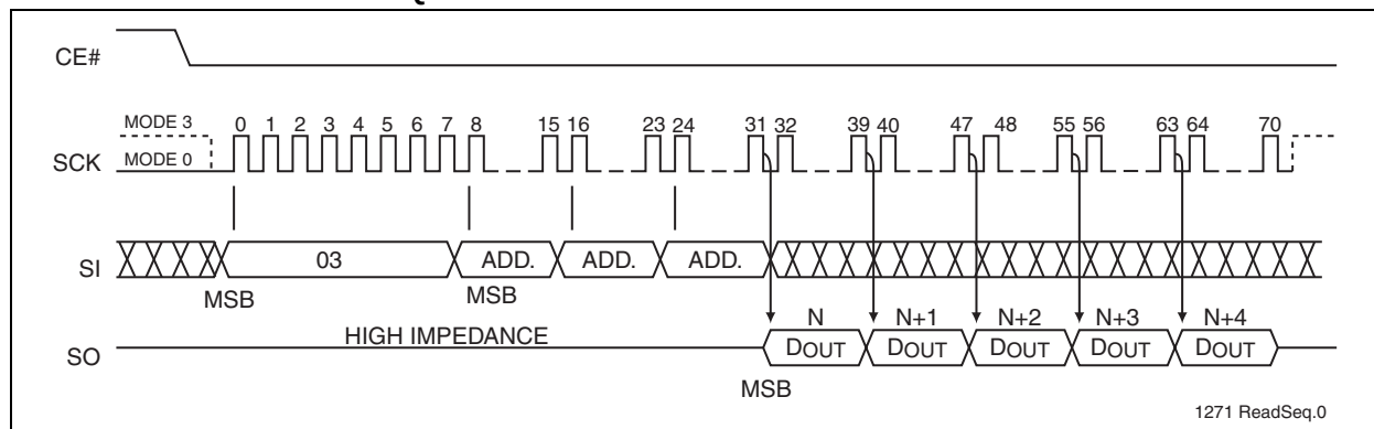
FIGURE 4-3: READ SEQUENCE
