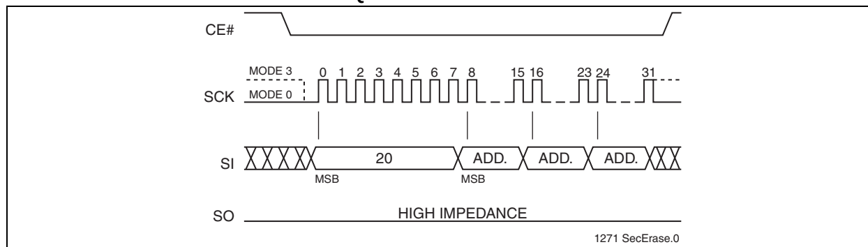
FIGURE 4-10: SECTOR-ERASE SEQUENCE
