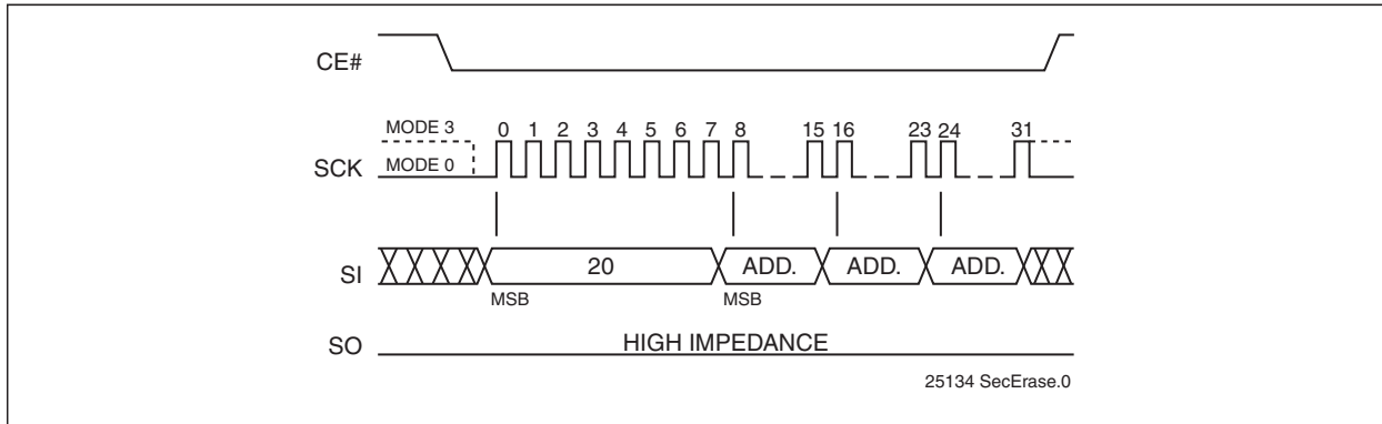
FIGURE 4-10: SECTOR-ERASE SEQUENCE
