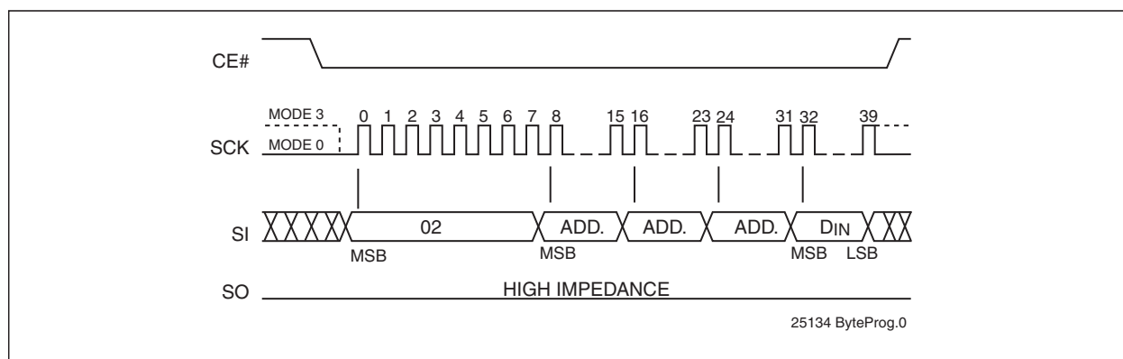
FIGURE 4-5: BYTE-PROGRAM SEQUENCE
