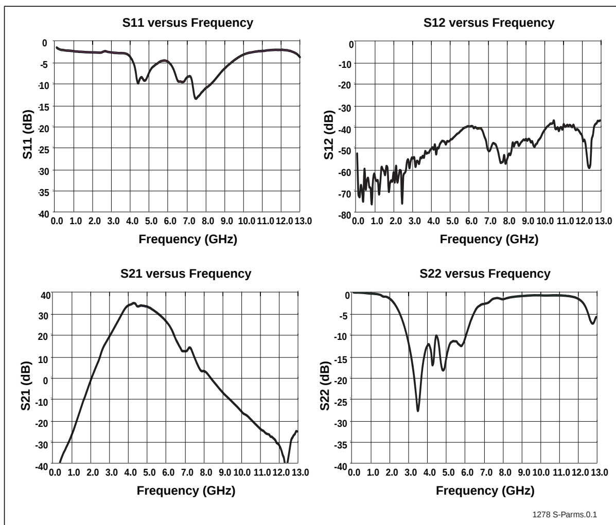
Figure 3: S-Parameters
