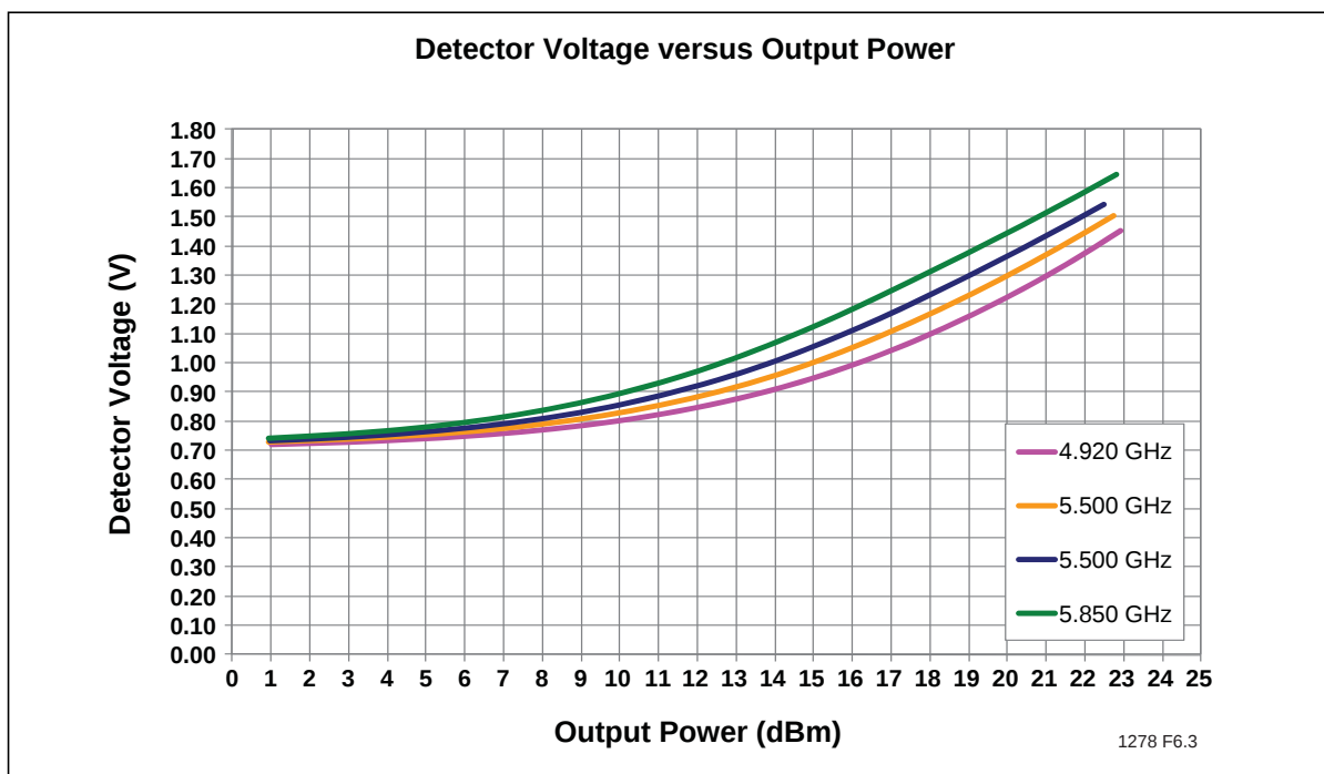
Figure 6: Detector Voltage versus Output Power
