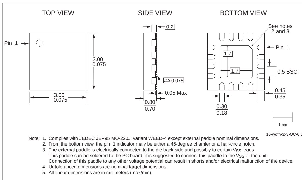
Figure 10: 16-contact Very-thin Quad Flat No-lead (WQFN) SST Package Code: QC
