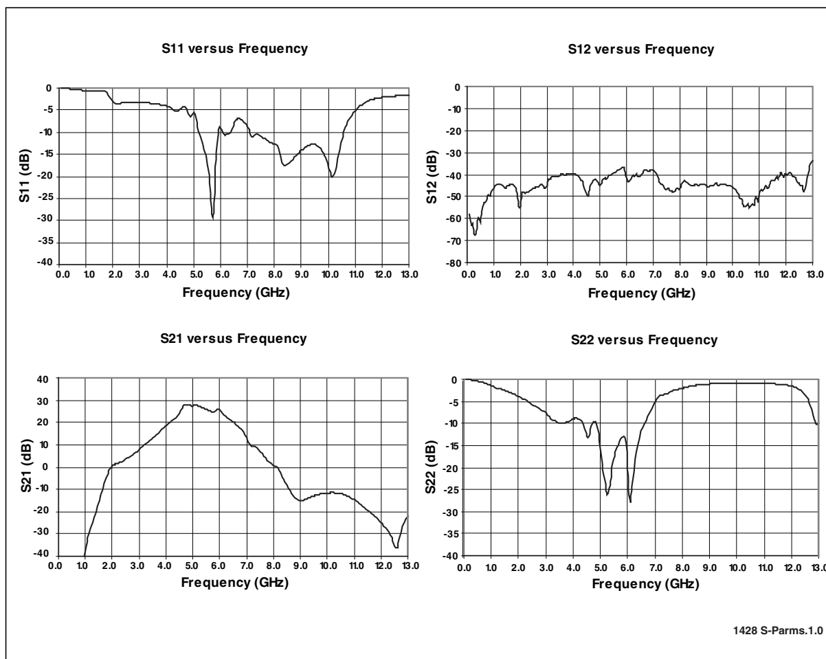
Figure 12: S-Parameters
