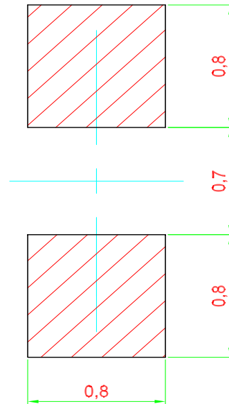
Alternative Solder-pad Compatible to ChipLED 0603
