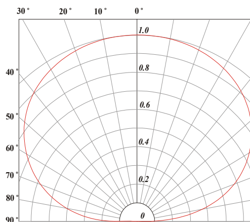
Radiation Pattern
